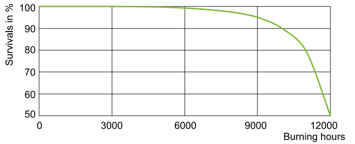
CDM-T 35W Life Expectancy /830, /842 G12
