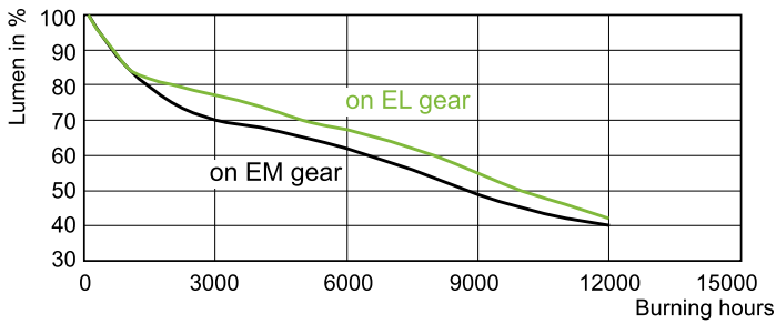
CDM-T 35W Lumen Maintenance /830
