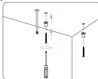
accessories drawing of suspending installation
