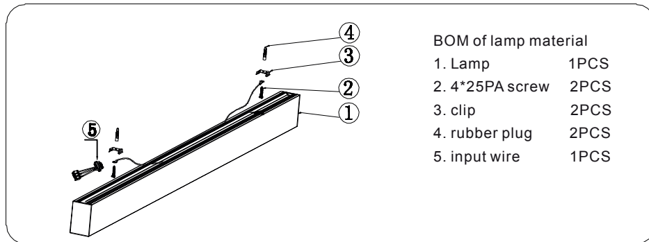
exploded drawing of ceiling installation
