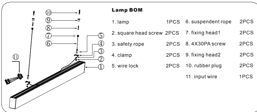
exploded drawing of suspending installation
