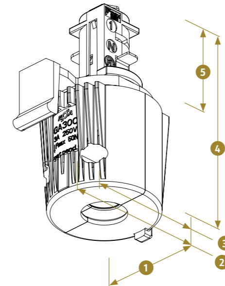
GA 300 1. 32 mm, 2. 44 mm, 3. 36 mm, 4. 62 mm, 5. 27 mm
