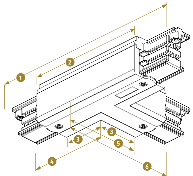
T-feed XTS 36, 37, 39, 40 1. 166 mm, 2. 100 mm, 3. 34 mm, 4. 67 mm, 5. 66 mm, 6. 99 mm
