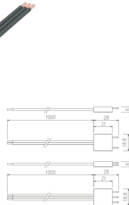
■ Power Plug 2Pins/3Pins Model number: TR4U12(2pins) Model number: TR4U13(3pins)
