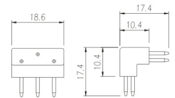
■ 3D Corner Pins Model number: TR4U08
