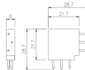
■ 2D Corner Pins Model number: TR4U07
