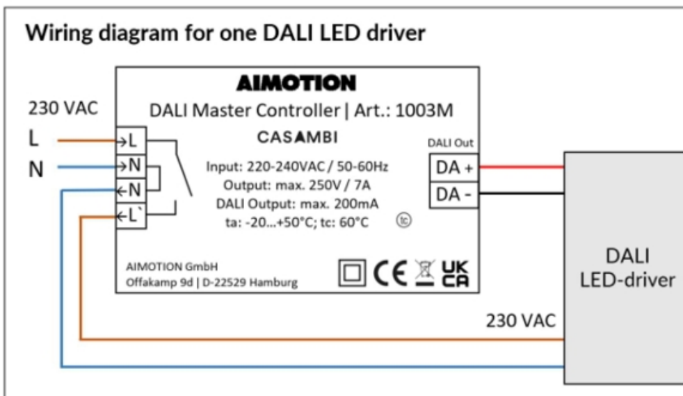
Wiring diagram with external relay, for multiple DALI LED drivers
